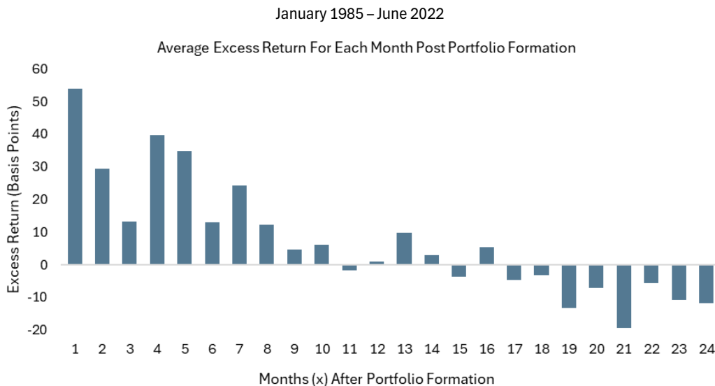
Figure 1: Buy & Hold Momentum Signal Decay Through Time
