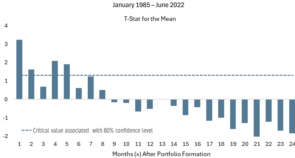
Figure A1.2: Fama-French Three-Factor Intercept Significance
