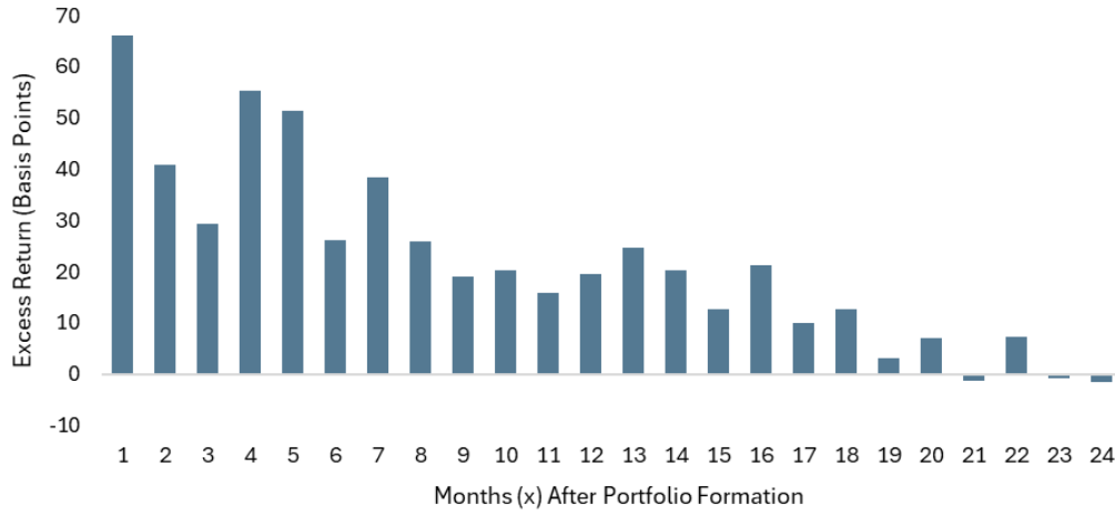
Figure A1.4: Fama-French Five-Factor Intercept Significance
